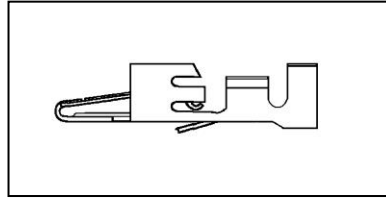
Figure 7.3 Turn Signal Connector Terminal
