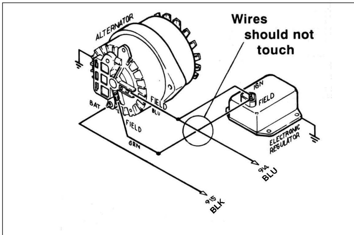
Figure 7-1A Mopar Alternator
