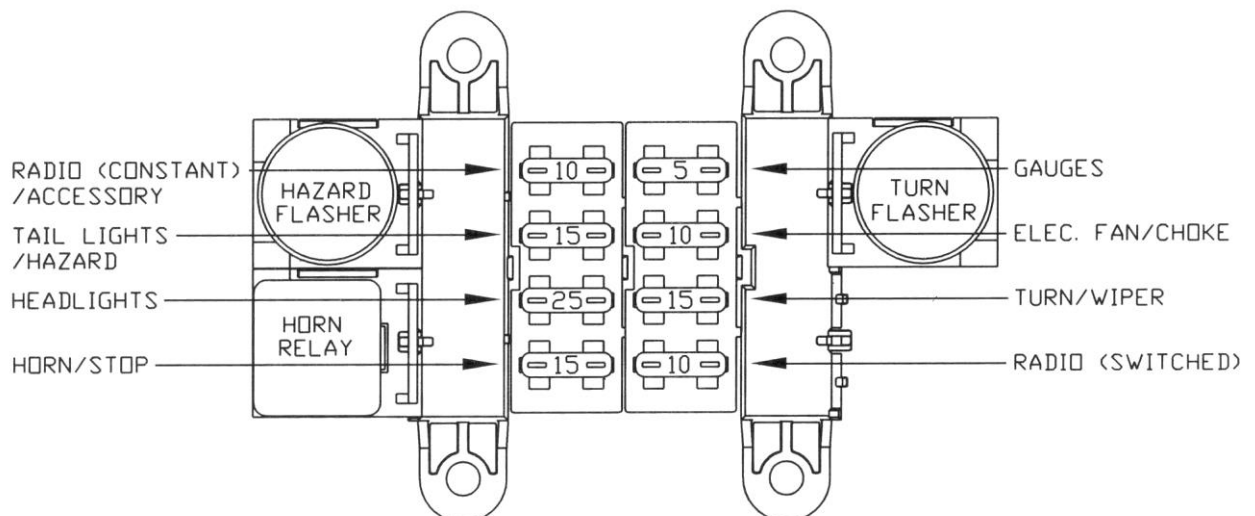
Figure 11-1 Fuse Requirements
