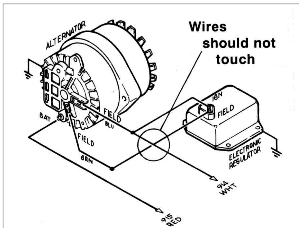
Figure 9-1A Mopar Alternator
