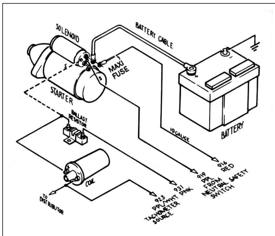
Figure 7-4 GM Ignition (Start-Run) System
