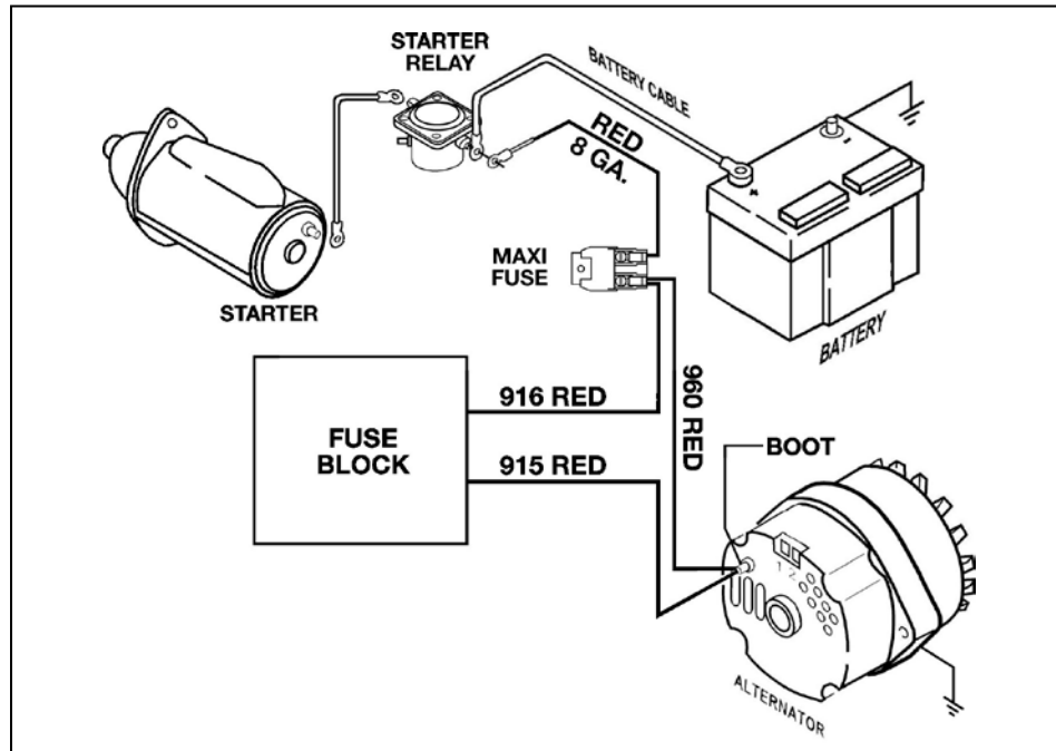
Figure 8-1B High Output Wire
