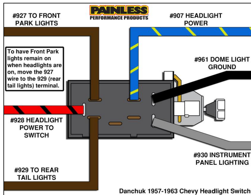
Figure 12-2 Headlight Section B 1957 Chevrolet Switch (Some Applications).
