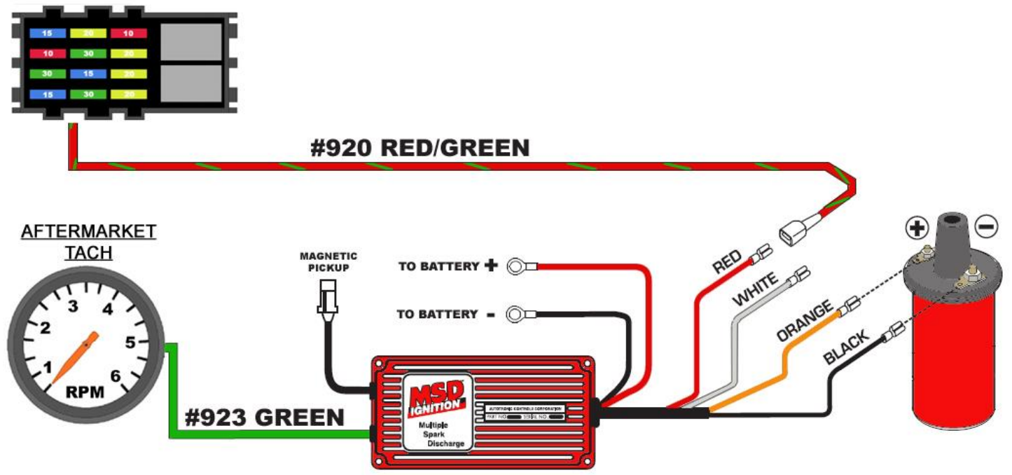
Figure 15 MSD Connections
