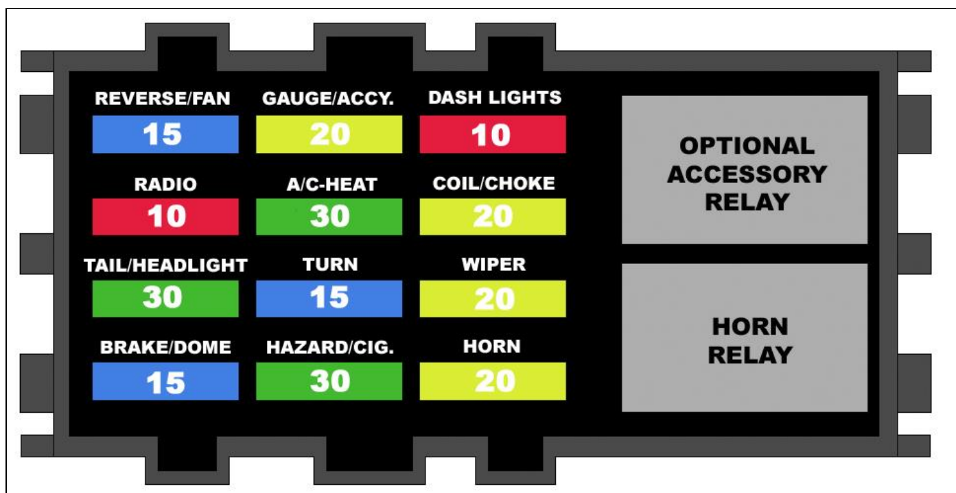
Figure 33 Fuse Requirements
