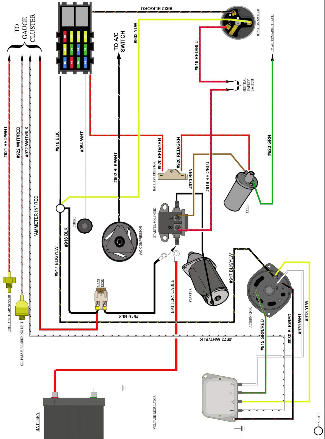
Figure 10 Engine Wiring
