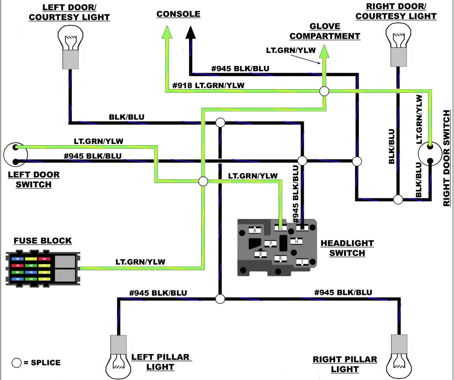
Figure 18 Interior Lighting Schematic Brake Light Switch
