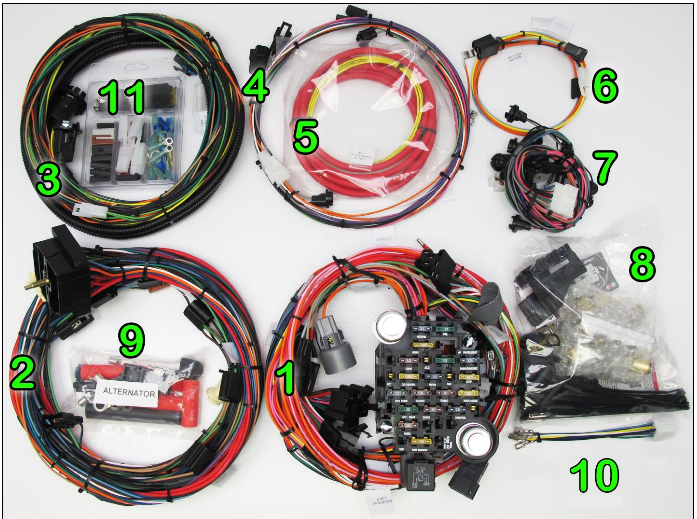
CONTENT FIGURE- All of the parts in the Painless kit
