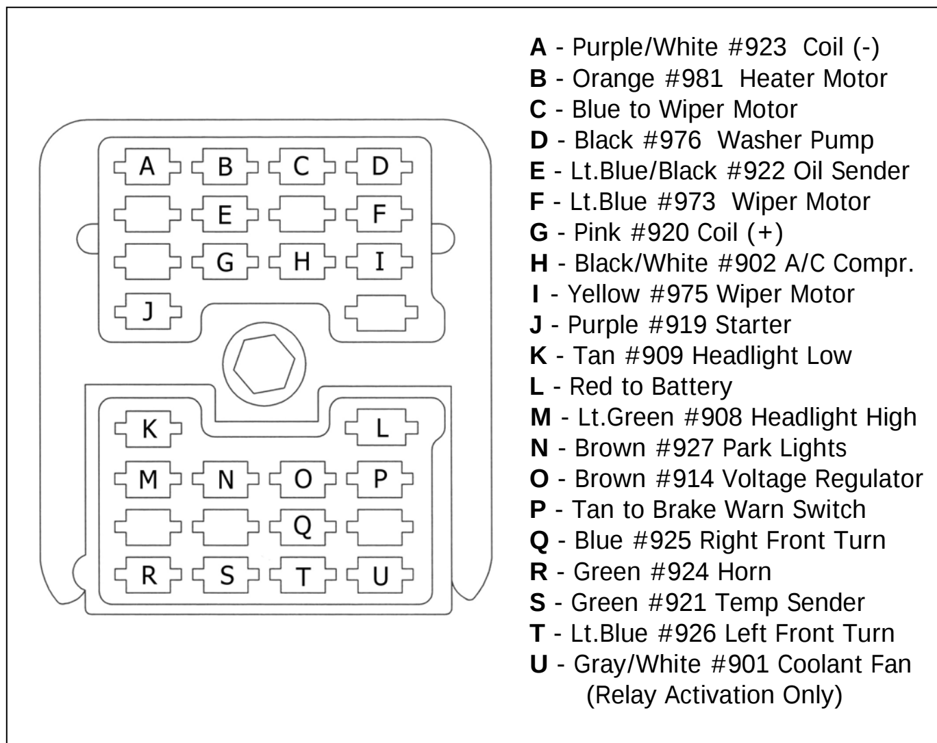
Illustration 1 Engine Harness Firewall Connector Style #1 (obsolete older style)
