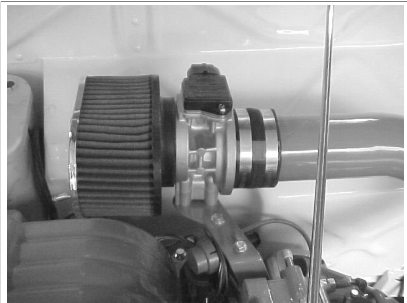
Figure 6.8 (MAF) Mass Air Flow Sensor w/air filter
