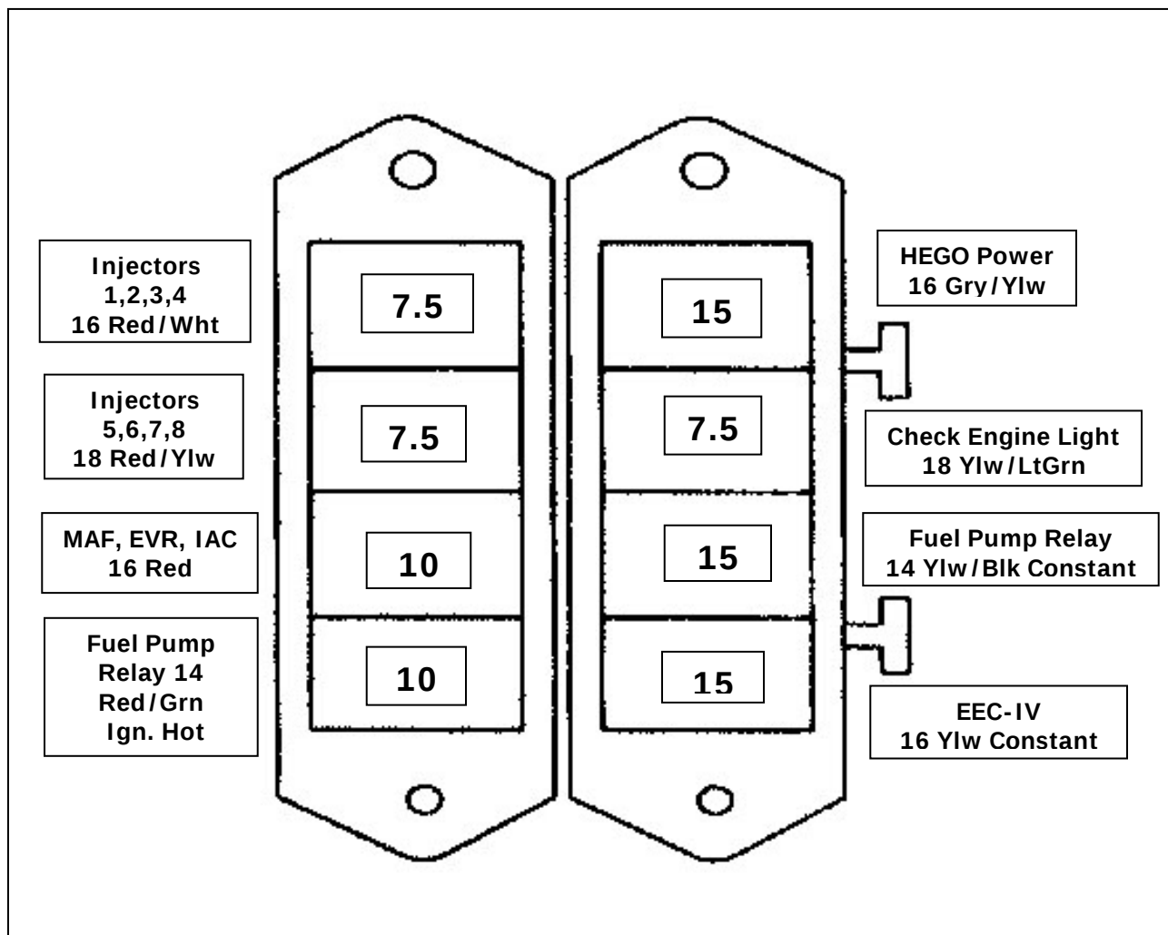
Figure 8.2 Fuse Location
