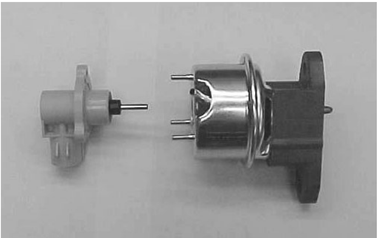
Figure 6.6 (EGR) Exhaust Gas Recirculation Valve
