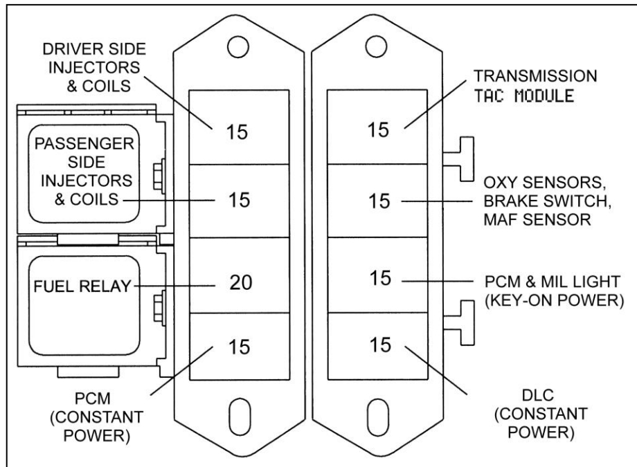
FIGURE 7.1 60522-23 Fuse Identification
