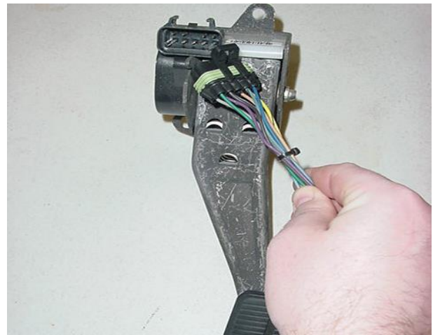
FIGURE 6.16 Accelerator Pedal
