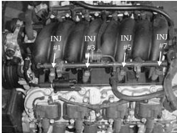
FIGURE 6.13 Injectors 1, 3, 5, 7
