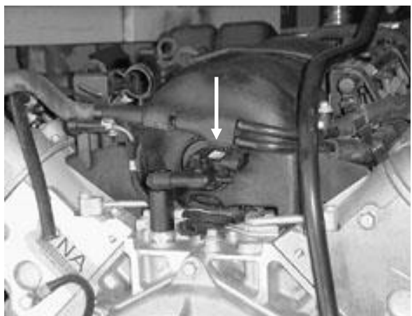
FIGURE 6.10 Map Sensor
