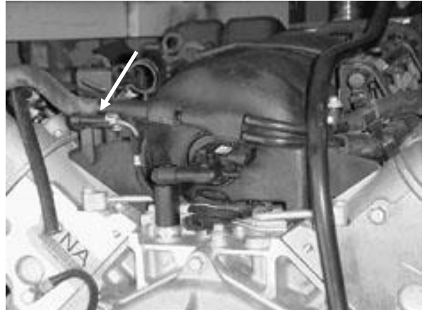
FIGURE 6.8 Knock Sensor Connector
