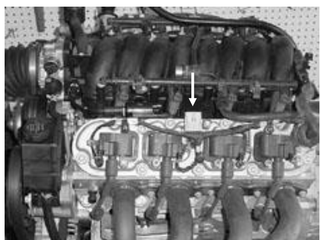
FIGURE 6.18 Driver Side Coil Connector
