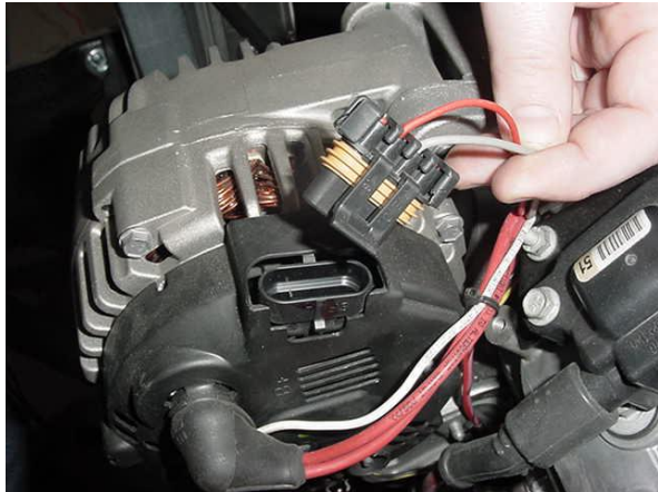
FIGURE 6.7 Alternator
