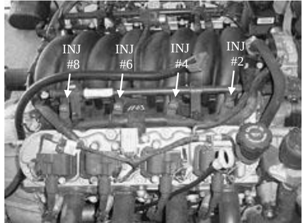
FIGURE 6.14 Injectors 2, 4, 6, 8
