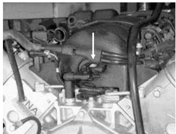
FIGURE 6.10 Map Sensor
