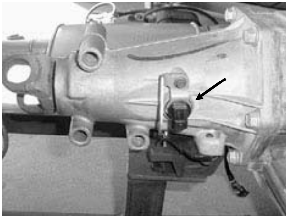
FIGURE 6.23 VSS (4L60E)
