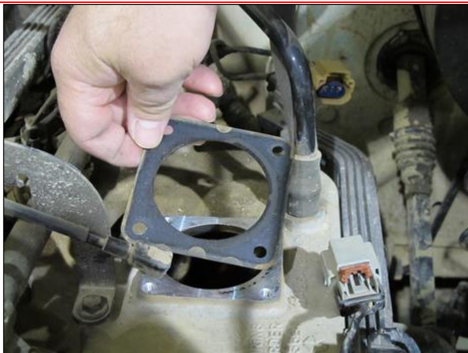
(Figure 3-12) Remove the old gasket from the intake manifold.
