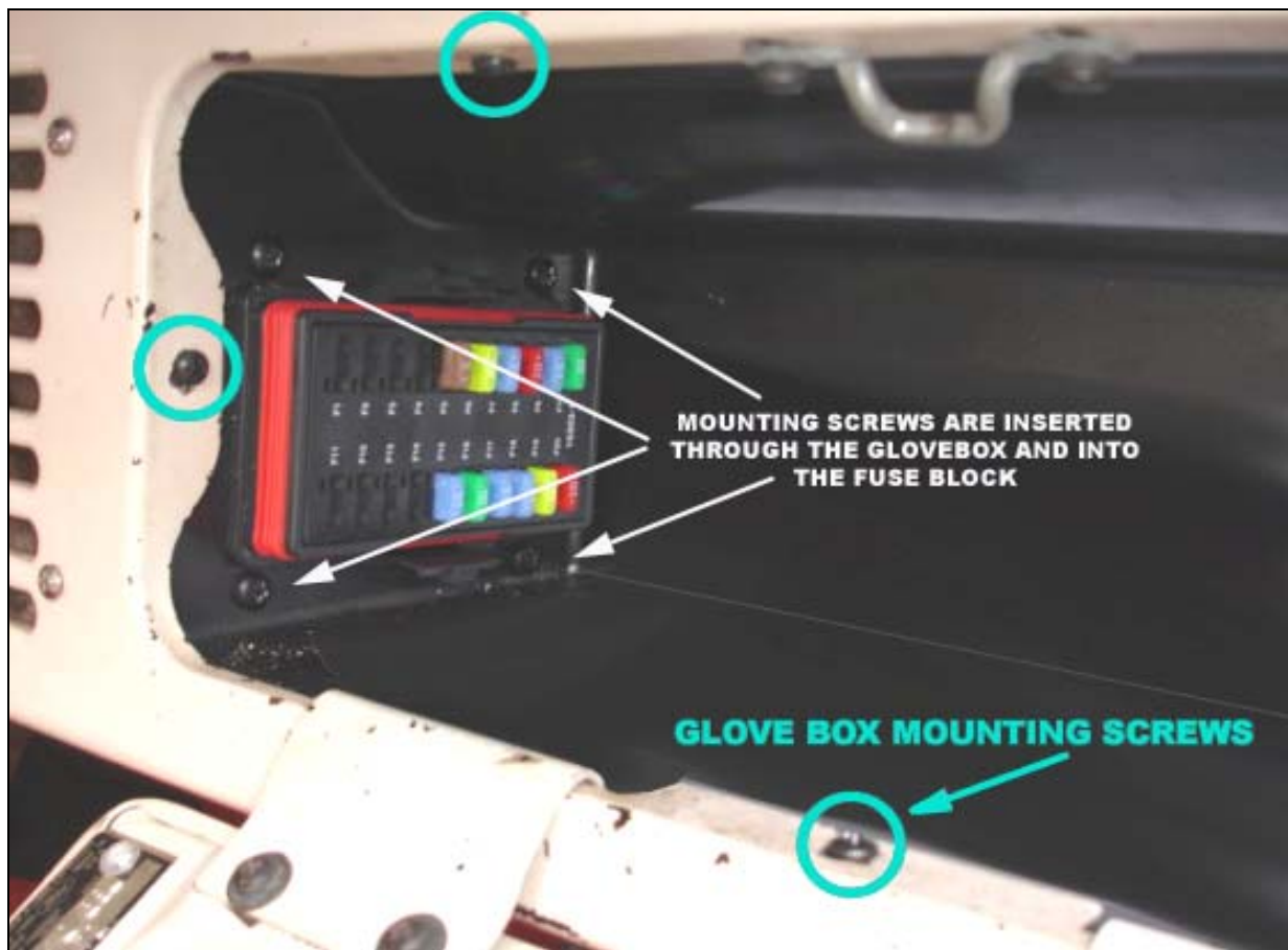
FUSE BLOCK MOUNTING
