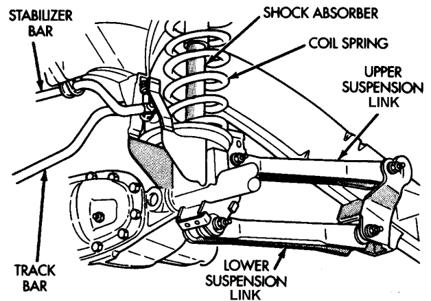
Upper and Lower Suspension Arms
