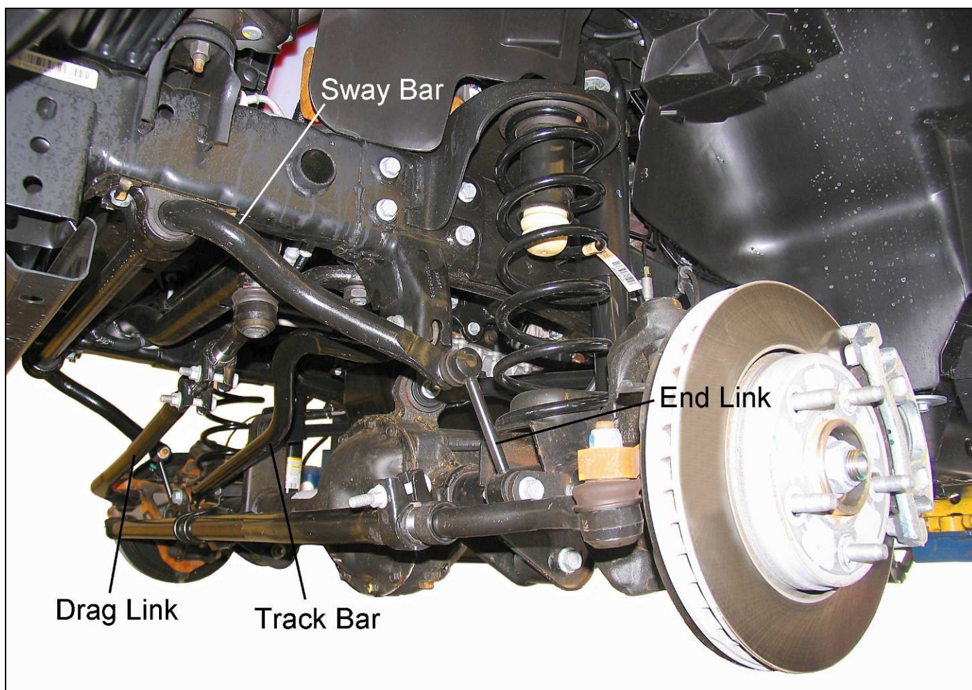
Front Suspension
