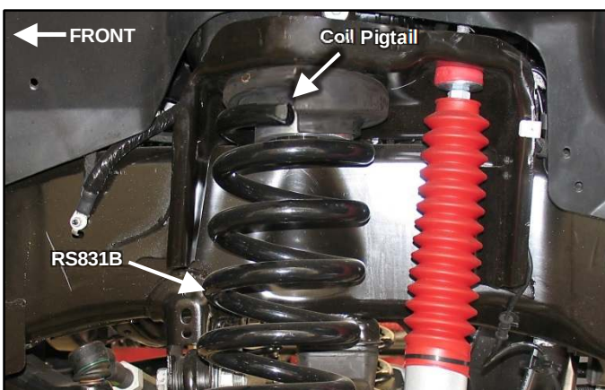
Driver side coil spring after rotating 90° from OE position Illustration 19
