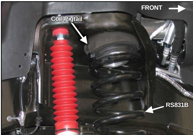
Passenger side coil spring after rotating 90° from OE position Illustration 18
