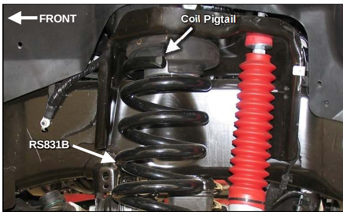
Driver side coil spring after rotating 90° from OE position Illustration 17
