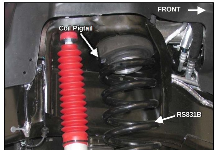
Passenger side coil spring after rotating 90° from OE position
