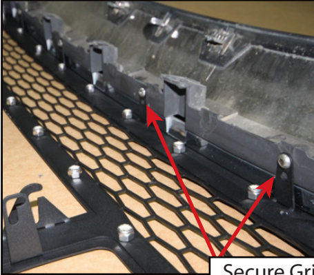
Secure Grille Pieces to Shell with 1/4" Bolts/Nuts
