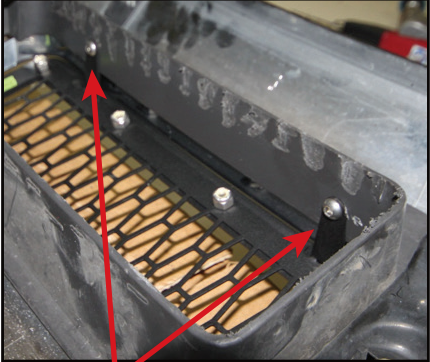
Secure Grille Pieces to Shell with 1/4" Bolts/Nuts
