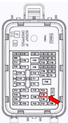
2024-2025 F-150 Fuse Block
