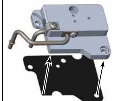
Figure 7 Gasket Installation onto Manifold
