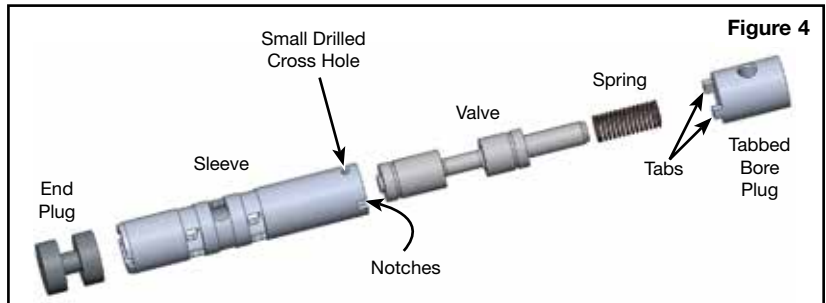
Valve Assembly Installation into Valve Manifold
