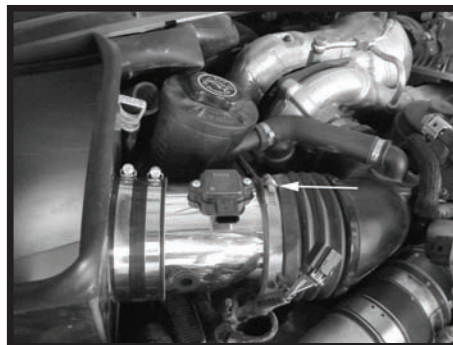
Step 12 Install the intake tube into the vehicle, position it as shown and once tube is in desired location fasten securely.
