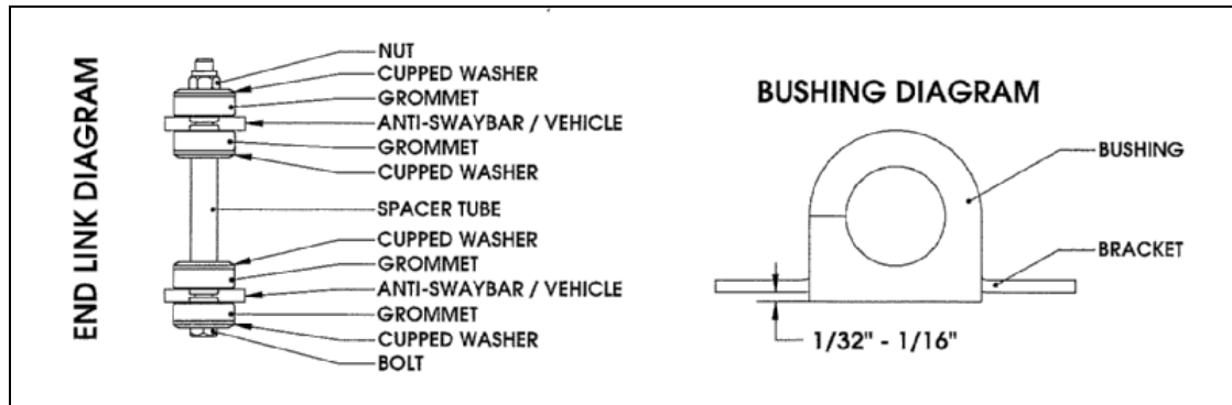
END LINK DIAGRAM
