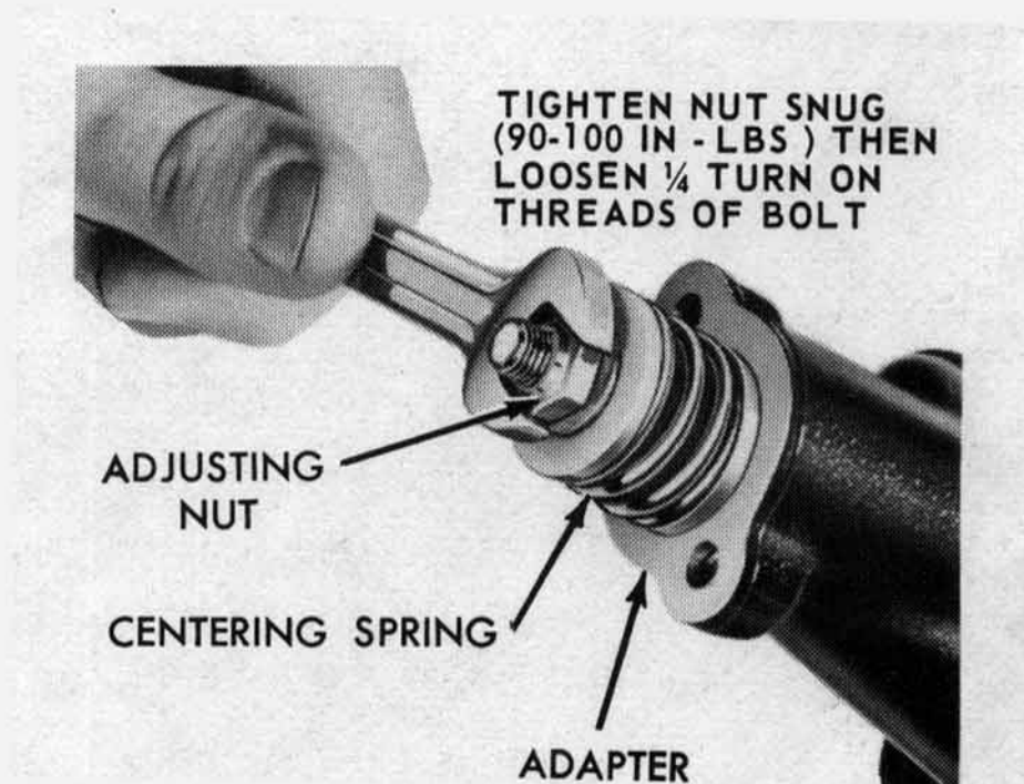
Figure 1a - Adjusting Center Spring
