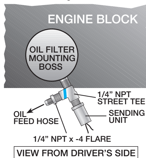
Fig. 3-b / View From Driver's Side ('99-'00 Models Only)
