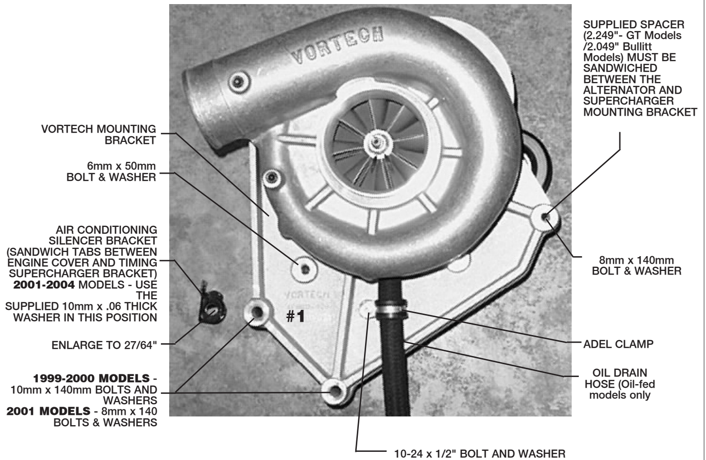
Fig. 8.2-d / Supercharger-Front View
