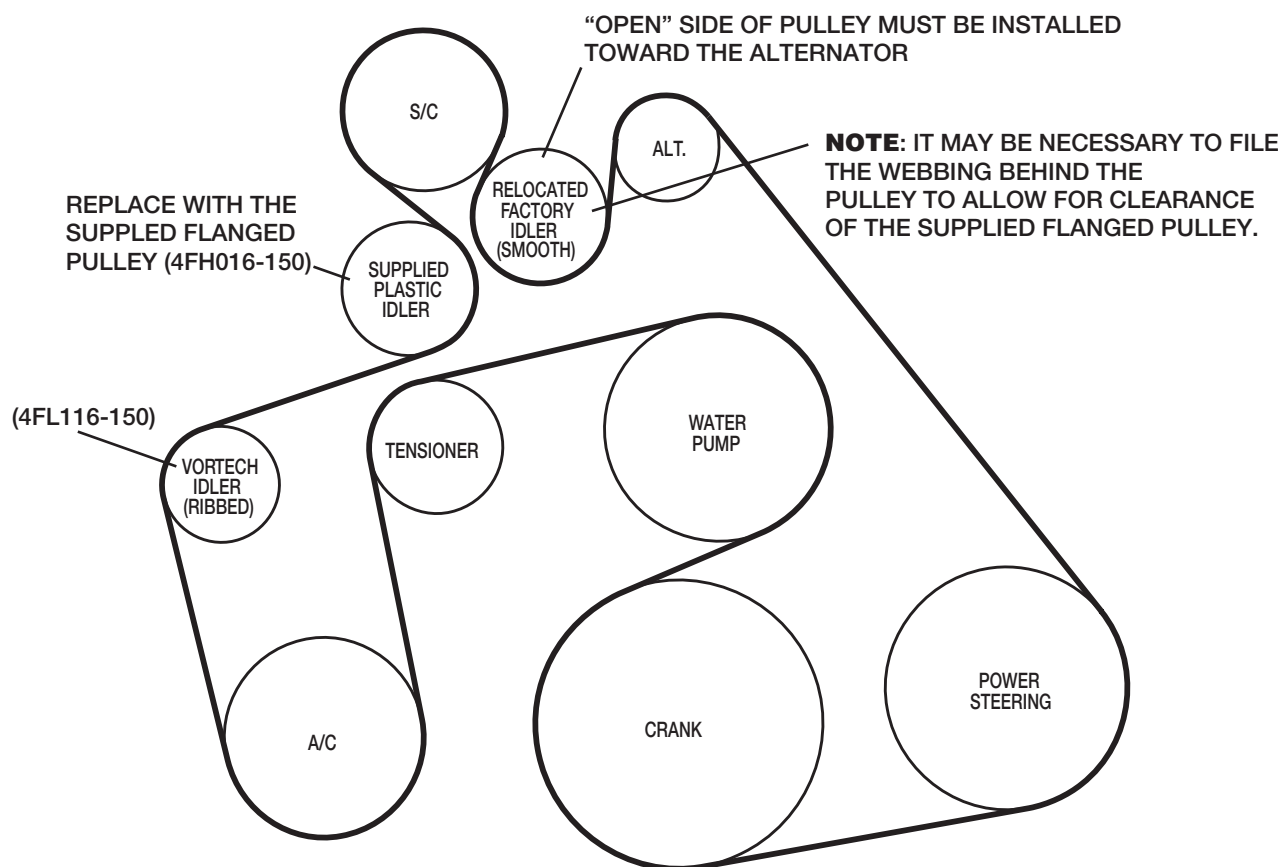
Fig. 8.2-f / Belt Diagram
