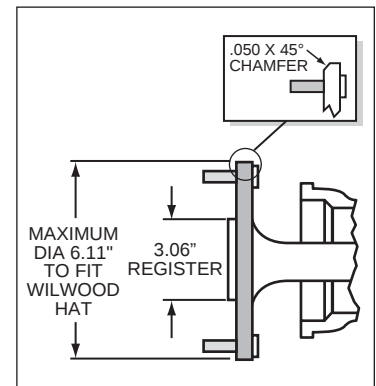
Figure 5. Axle Flange Maximum Dimension
