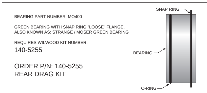
Figure 2. Loose Fit Bearing Configuration
