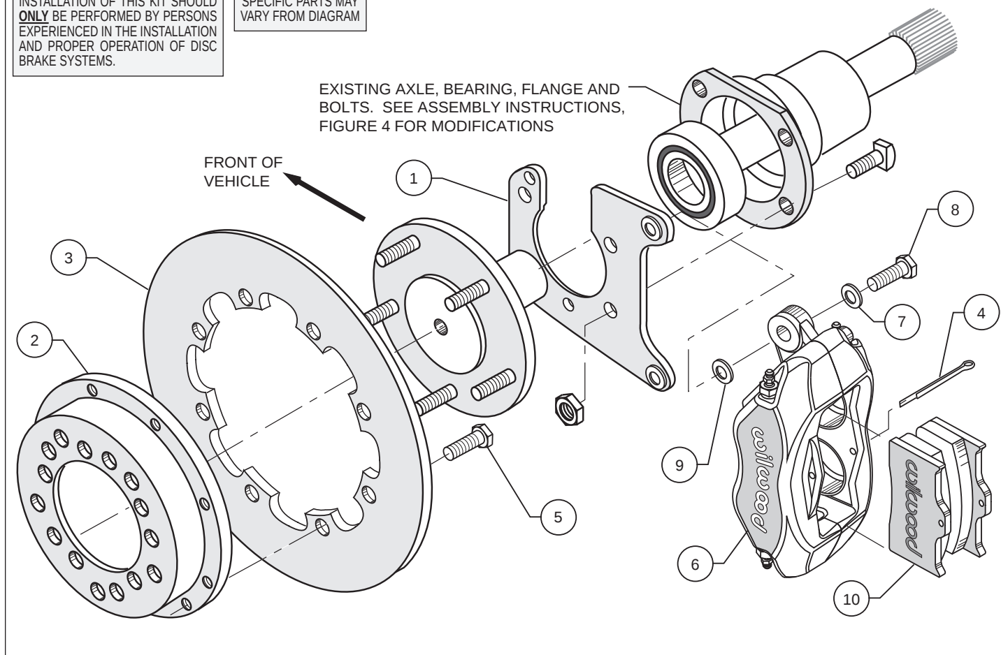
Figure 4. Typical Installation Configuration
