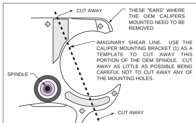
Figure 2. Stock Spindle Modifications
