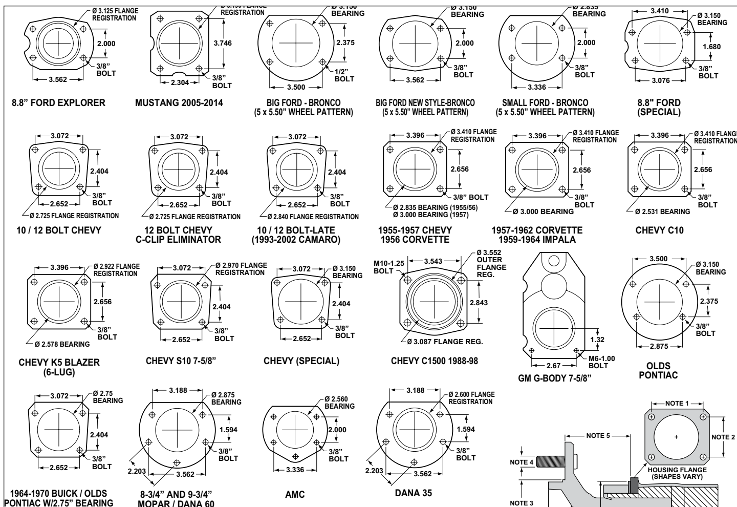
Figure 4. Rear Housing Flange Chart and Axle Flange / Offset Cross-Section
