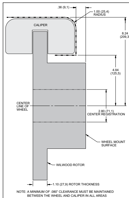
Figure 3A, P/N 140-15845. Wheel Clearance Diagram
