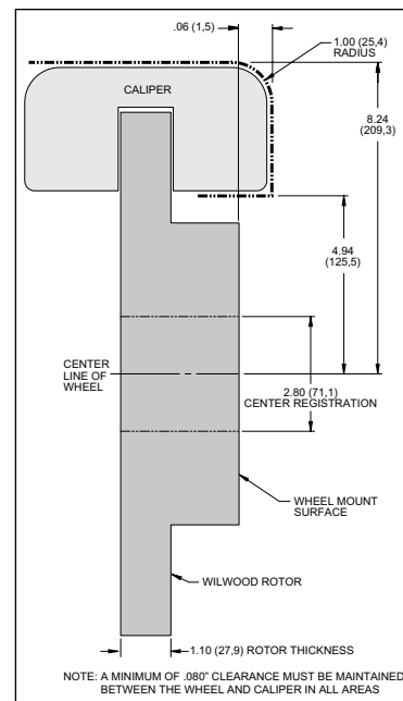
Figure 3B, P/N 140-16132. Wheel Clearance Diagram
