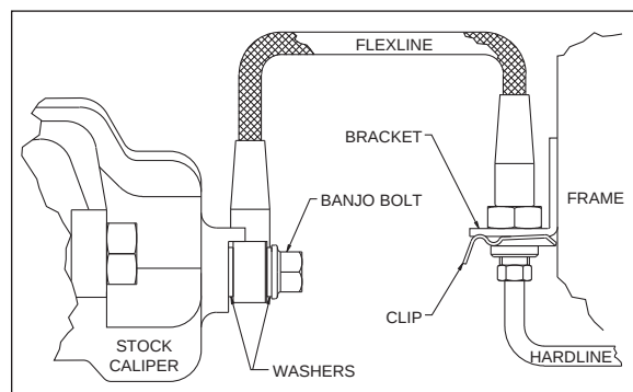
Figure 3. Brake Line Diagram
