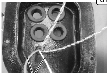
Route heavy gauge orange and white wires through 7/8" wiring grommet on kick panel
