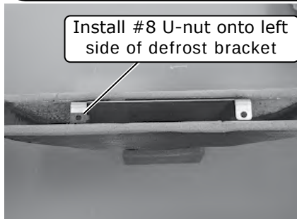
Driver-Side Defrost Duct
