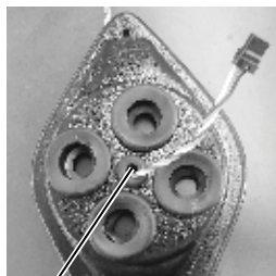
Route main wiring harness (white/yellow/purple) through wiring grommet on fresh air cap
