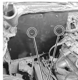
Using full-length studs locate upper mounting holes in firewall
