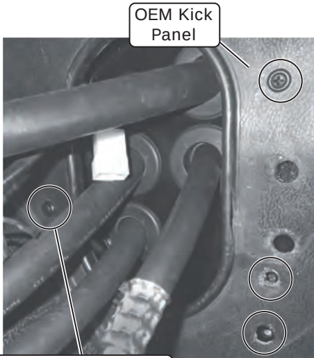
(4) #8 x 1 1/4" Countersunk Screws with Washers
