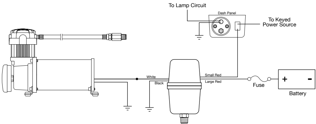
Wiring Diagram: (Figure 2)
