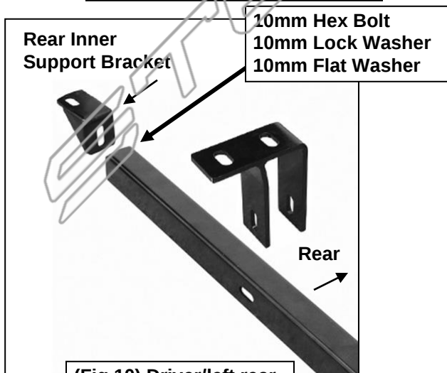
(Fig 10) Driver/left rear Bracket assembly
