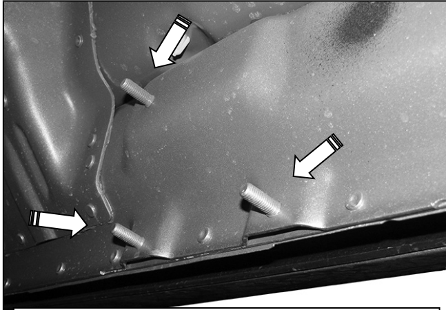
(Fig 1) Locate the (3) factory threaded studs at each location. Passenger side rear pictured
