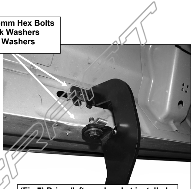
(Fig 7) Driver/left rear bracket installed
