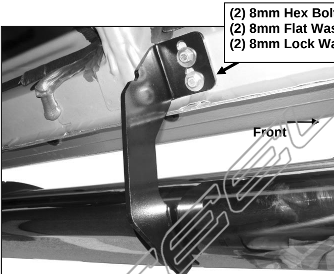
(Fig 3) Driver side center mounting location pictured
