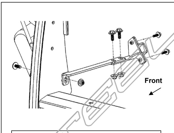
(Fig 16A) Passenger side Top Outer Bracket pictured installed in "top position"
