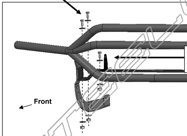
(Fig 13) Passenger side Cross Bar Light Mount installation illustrated
