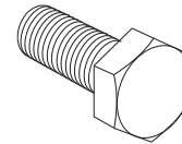
Hex Bolt 12mm x 35mm Part # 3006097 Qty 3
