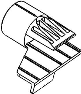
Plastic End Caps Qty. 2 Part # 592.66 RH Part # 593.71 LH
