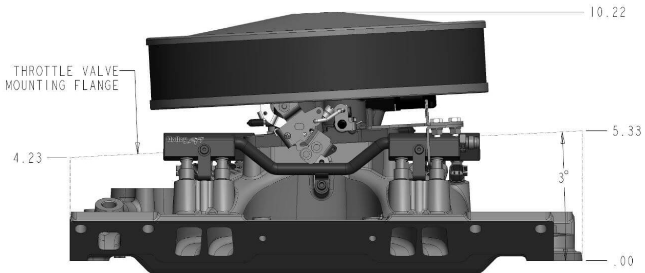
300-263 SHOWN WITH 112-587 THROTTLE VALVE AND 120-102 14" AIR CLEANER
