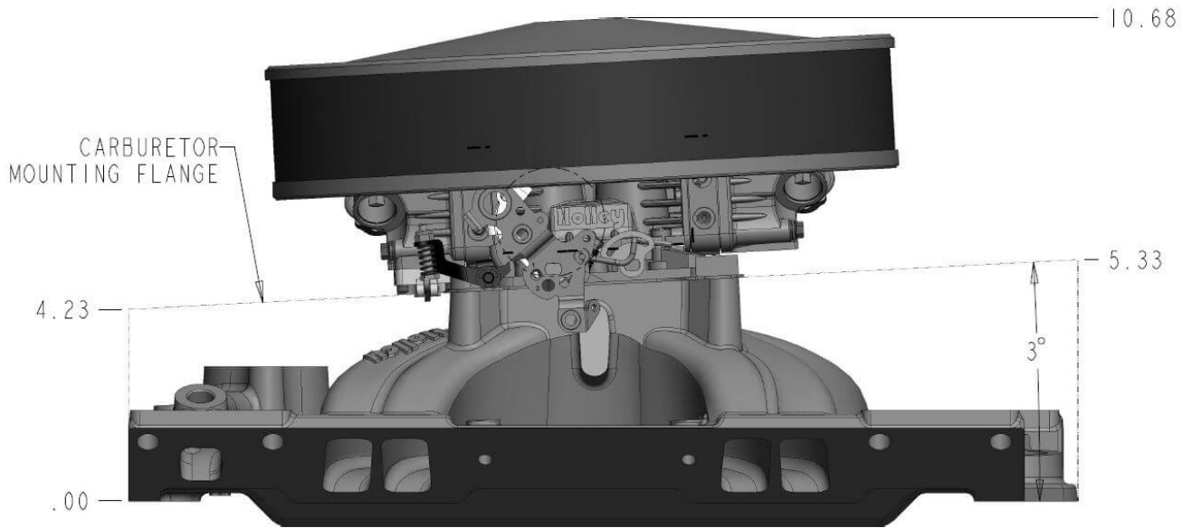
300-264 SHOWN WITH 4150 CARBURETOR AND 120-102 14" AIR CLEANER
