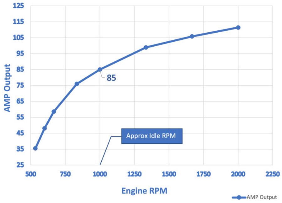
Typical Performance @ 12.8 Volts
